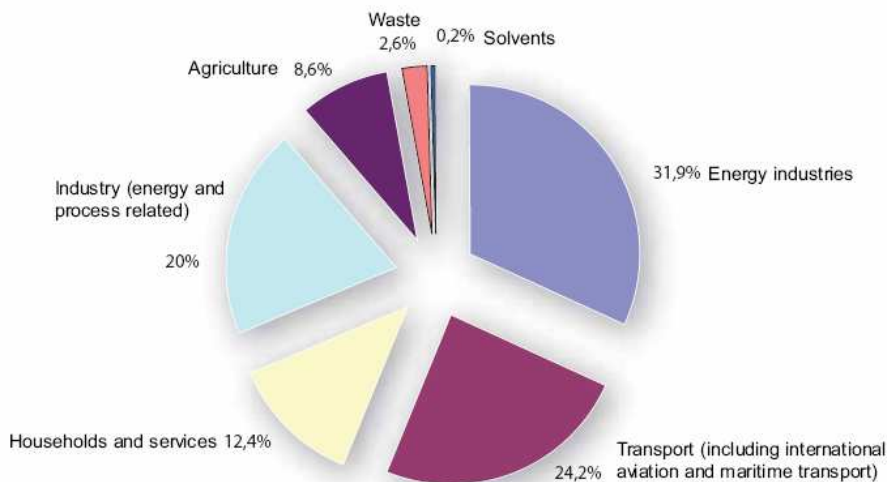
Total EU-27 greenhouse gas emissions by sector, 2007
